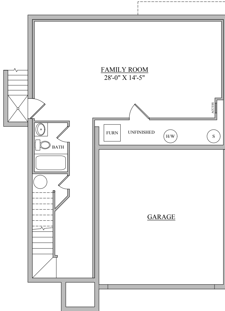
FINISHED BASEMENT PLAN BEECHWOOD
