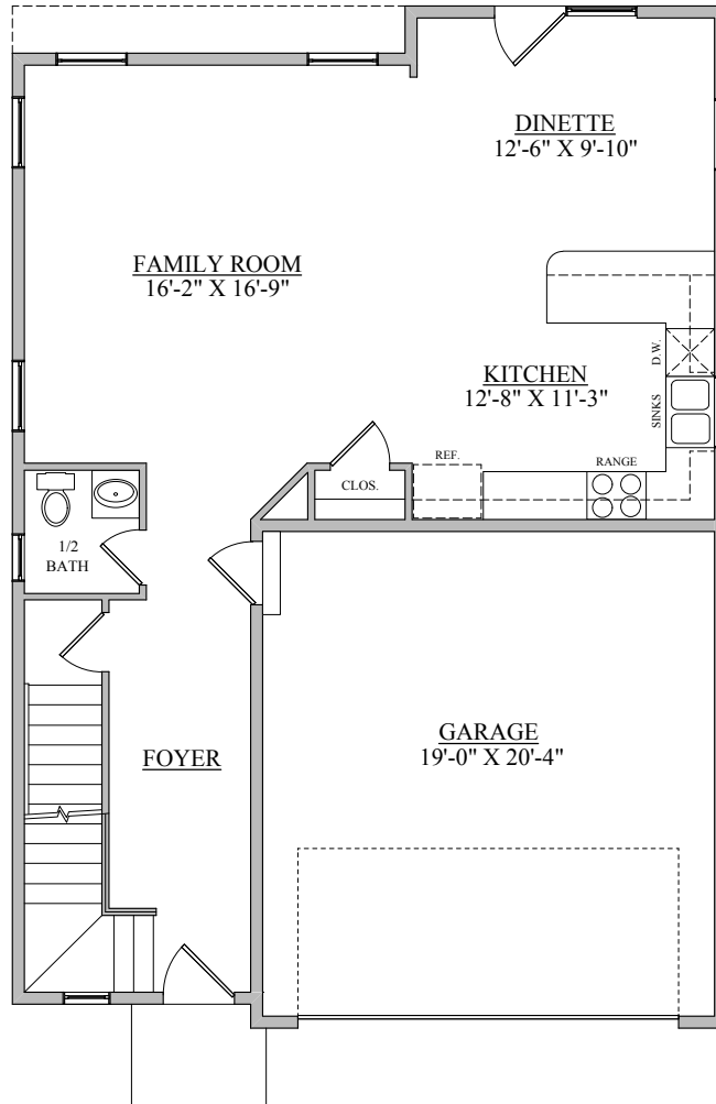
FIRST FLOOR PLAN BEECHWOOD
