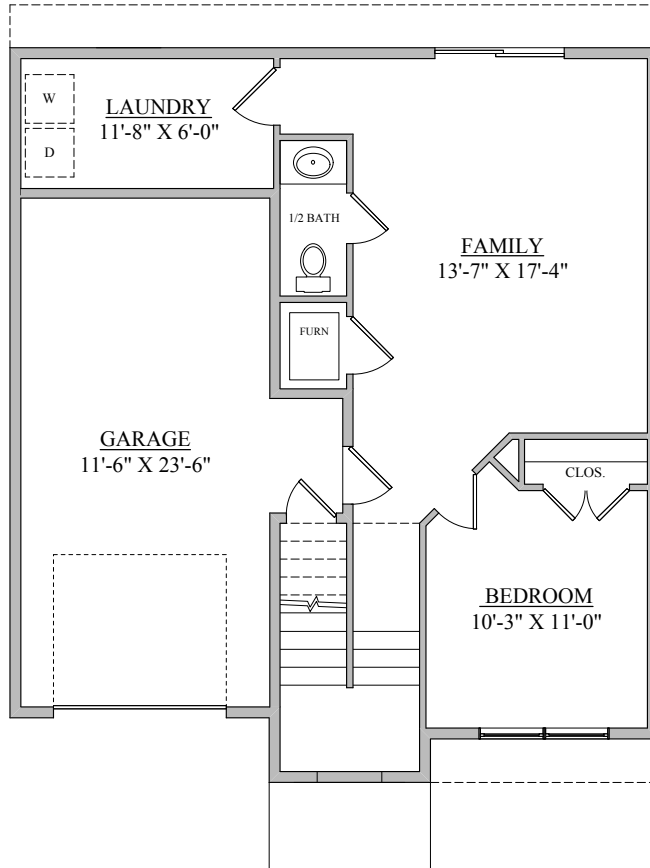
LOWER FLOOR PLAN MAGOTHY
